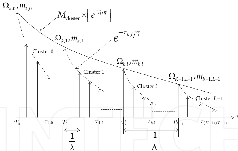
Fig. 3. Temporal model of IEEE 802.15.4a UWB Channel
