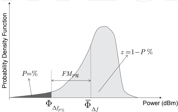
Fig. 13. Fade margin in UWB channel
