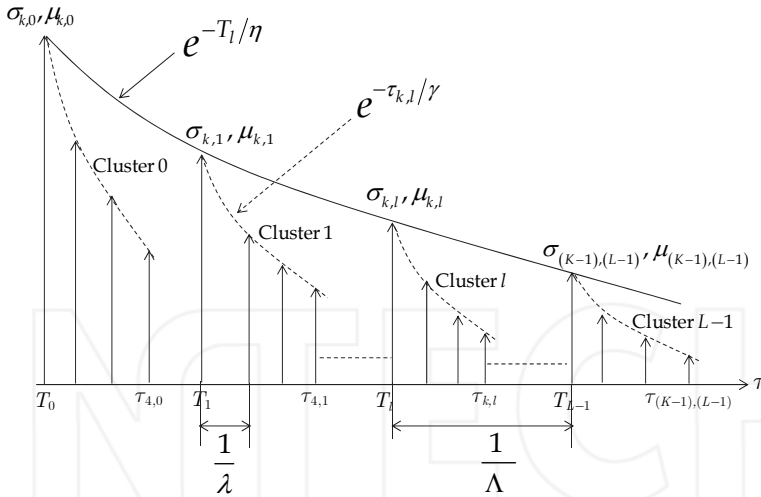
Fig. 2. Temporal model of IEEE 802.15.3a UWB Channel
