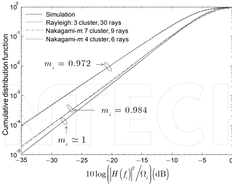
Fig. 5. Cumulative distribution function of the normalized channel frequency amplitude |H(f_i)| , using the Nakagami- m analytical approximation, for several MPC contributions.
